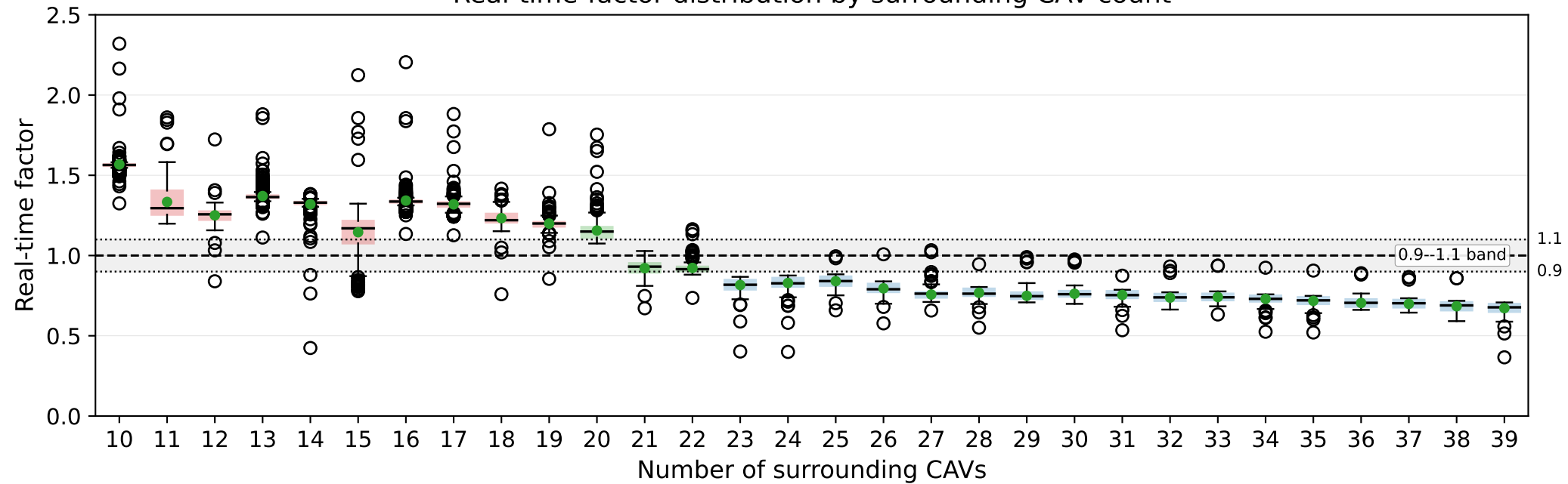
Real-time-factor distribution by surrounding CAV count
